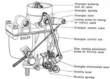
Fig. 13 Linkage between the strangler lever and the throttle lever
