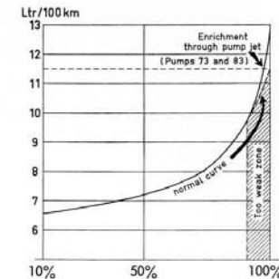
Fig. 39 Consumption curve of a vehicle on a level road with enrichment through the pump jet
