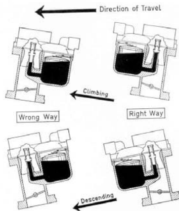
Fig. 4 Position of the Float Chamber
