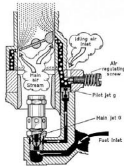
Fig. 17 Idling with air control
