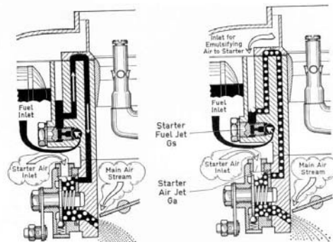
Fig. 7 Operation of the Starter Disc Valve
