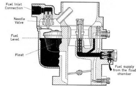
Fig. 6 The Float System
