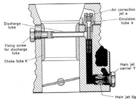
Fig. 28 Jet assembly of the 40 PII carburetor
