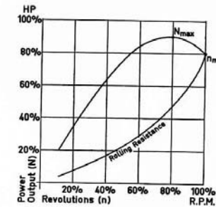
Fig. 1 Maximum Power Revolutions and Peak Revolutions
