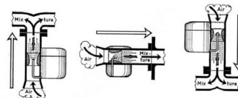
Fig. 2 Types of carburetor a) Upraight carburetor b) Horizontal carburetor c) Downraught carburetor
