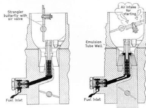
Fig. 14 Strangler Butterfly with Air Valve
