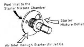
Disc Valve of a simple Starter
