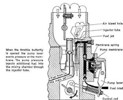
Fig. 33 Accelerator pump of the 28 PCI carburetor
