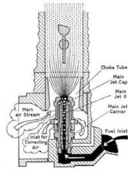
Fig. 20 Main jet circuit of a updraught carburetor
