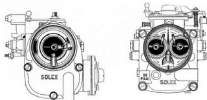
Fig. 3 Types of carburetors
