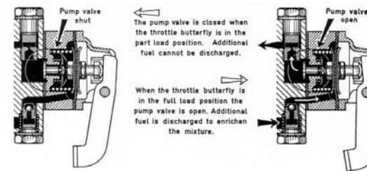
Fig. 35 "Rich" pump with disc valve (pump 83)
