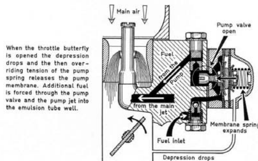
Fig. 30 Depression operated accelerator pump
