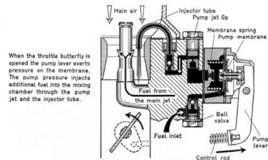
Fig. 29 Mechanically operated accelerator pump
