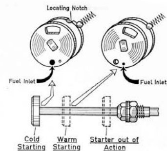
Fig. 9 Disc Valve and Starter Control of a Bi-Starter
