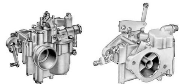
Type 32 HR (Horizontal Carburetor)
