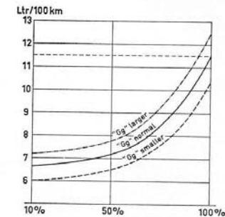
Fig. 21 Diagram of the effect of the main jet Gg
