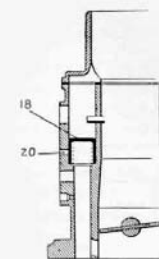
Fig 2 Starter in action (after starting)
