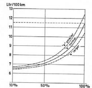
Fig. 22 Diagram of the effect of the air correction jet a
