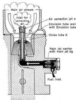
Fig. 19 Main jet circuit of a downdraught carburetor
