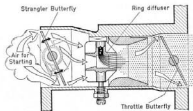
Fig. 15 Semi-Automatic Strangler
