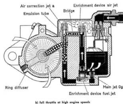
b) full throttle at high engine speeds
