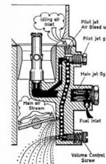
Fig. 16 Idling with mixture control
