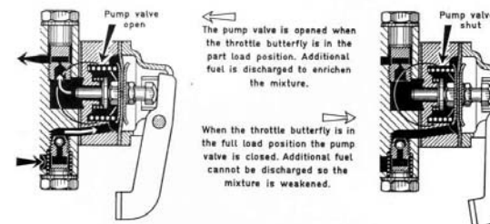
Fig. 36 "Weak" pump with disc valve (pump 84)
