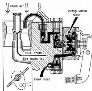
Fig. 34 "Rich" pump with ball valve (pump 73)
