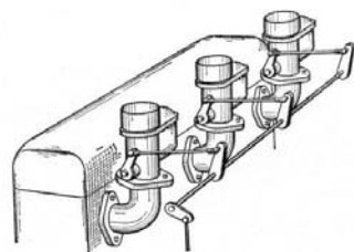
Fig. 5 Control layout for multiple carburetors
